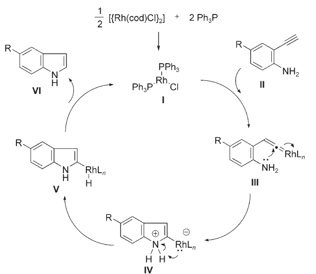
Scheme 3. Proposed mechanism of the cycloisomerization.
